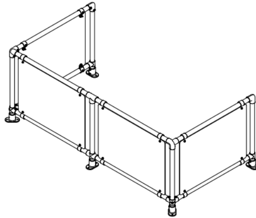
Figure 1: Example layout of a four-panel e-scooter corral.
